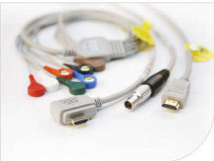
动态心电电缆与导联线系列 Holter Recorder ECG Patient Cable and Lead Wires
